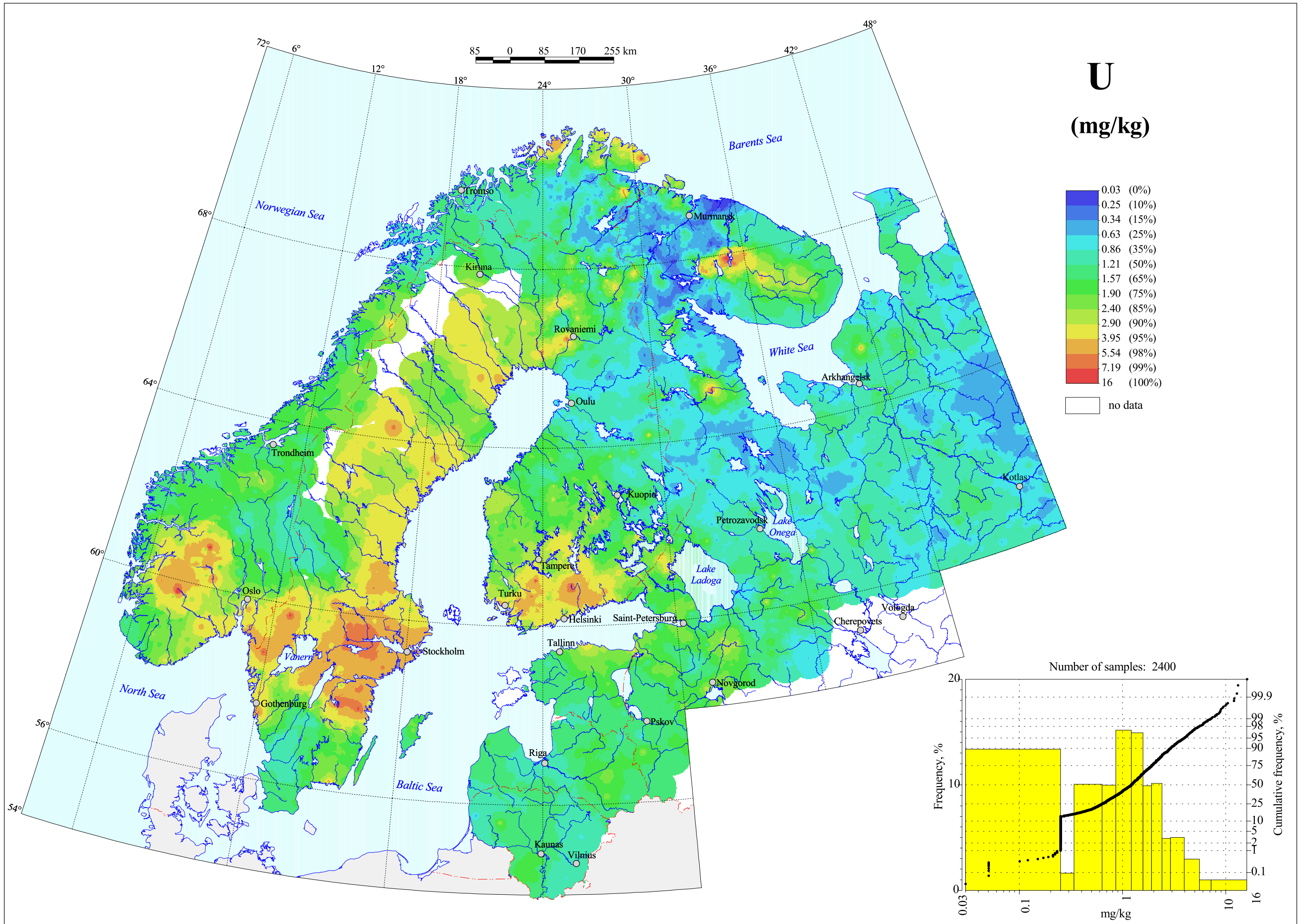
Uranium in C-horizon, Grain Size <2 mm, Total Content
